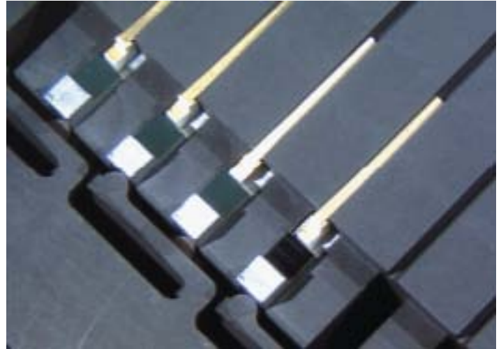
Graphite Fixture with Integrated Positioning Springs
